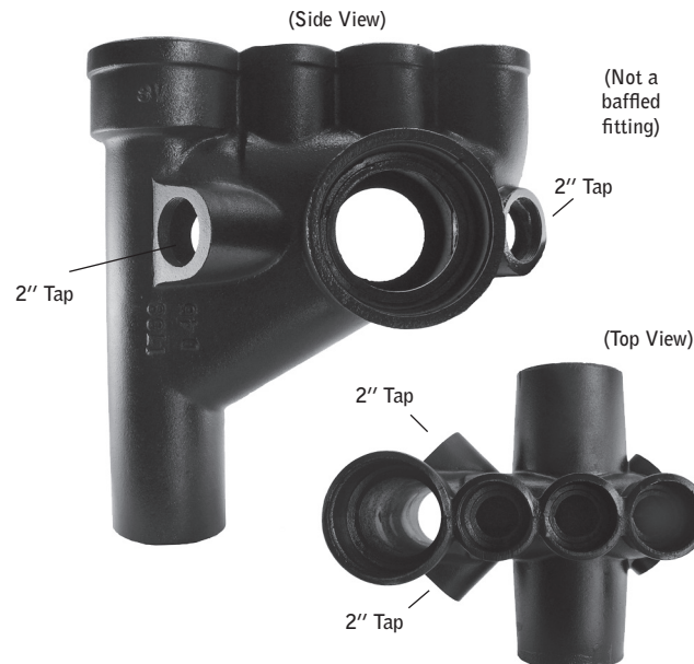
Part No. SV-1739 D Vented Closet Cross with 2" 45° Taps (Designed for use above the floor)
