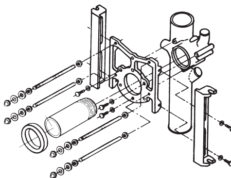
EZS 22 and EZS 24 Assemblies Illustrated
